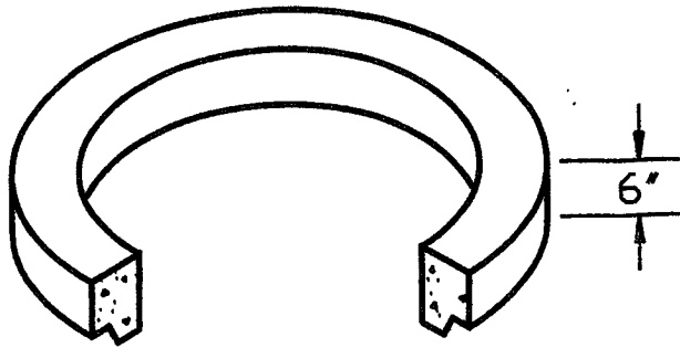
6" GRADE RING 210-50-75000
