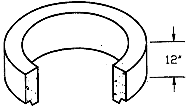
12" GRADE RING 210-50-75010
