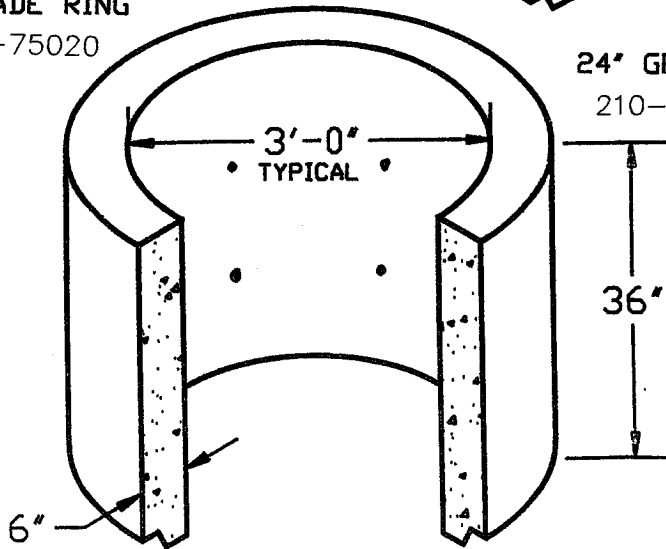
36" GRADE RING 210-50-75040
