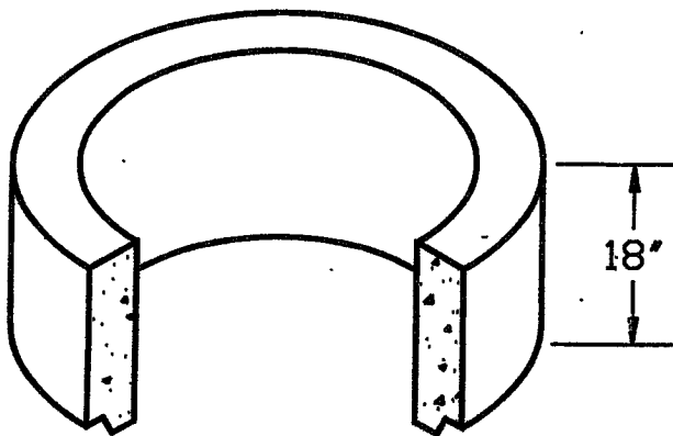
18" GRADE RING 210-50-75020
