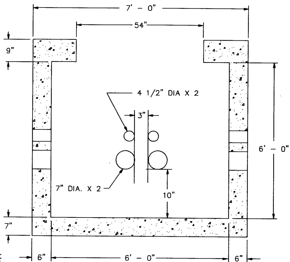
SECTION
